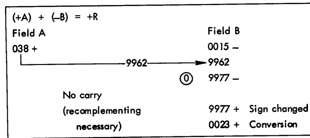
Figure 6. Complement Add with Recomplementing
