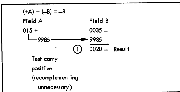
Figure 5. Complement Add with no Recomplementing
